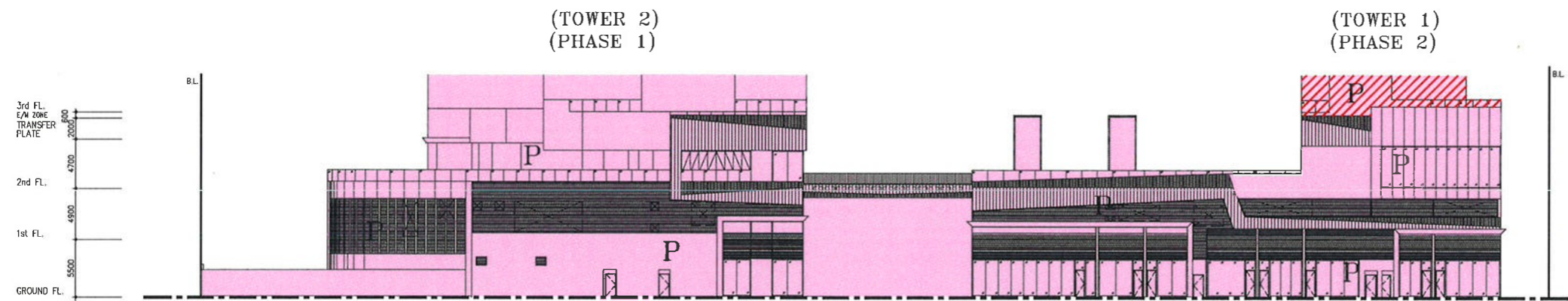
ELEVATION 8 PLAN
